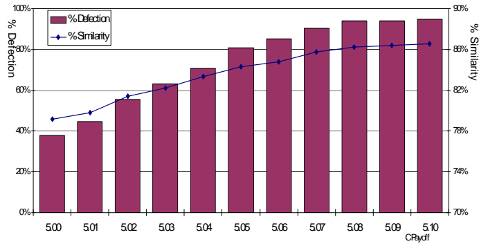
Figure 4: % Defection and % Similarity versus C Payoff in Combined Game, \phi = 1 .
