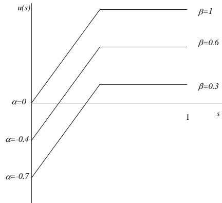
Figure 1: Utility versus segregation levels for different \alpha - \beta combinations.
