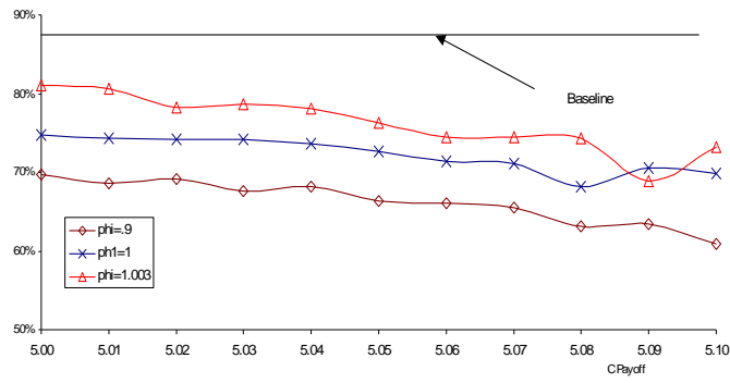
Figure 8: % Similarity versus C payoff for three different values of \phi , when the game ends in all-cooperate.
