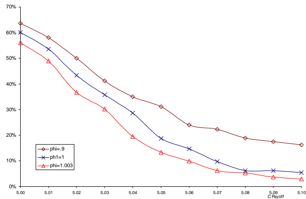
Figure 9: Welfare versus C payoff for different values of \phi .
