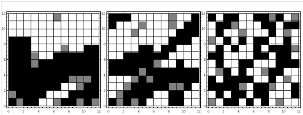
Figure 2: Three outcomes of the Schelling game for different \alpha - \beta combinations. Left: \alpha = -1, \beta = 0 . Middle: \alpha = -0.7, \beta = 0.3 . Right: \alpha = -0.2, \beta = 0.8
