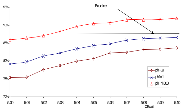
Figure 7: % Similarity versus C payoff for three different values of \phi .
