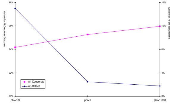
Figure 10: Welfare versus \phi , C = 5.01 .
