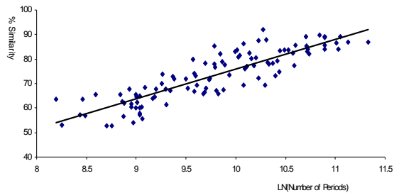
Figure 6: % Similarity versus number of periods till reaching an equilibrium, for the all-cooperate outcome. C = 5.05, \phi = 1 . The regression line is \widehat{\%Similarity} = -45.4 + 12.1Ln(\# \text{ periods}) . \# \text{ obs.} = 104, R^2 = 0.76 . Both coefficients are stat. sig. at greater than the 99% level.
