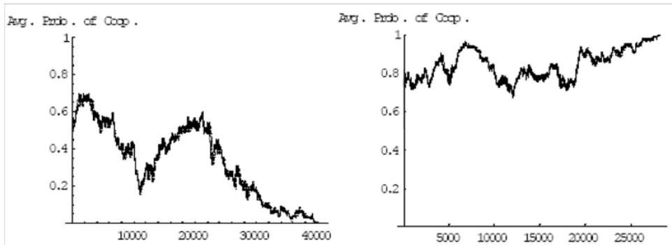
Figure 3: Two outcomes for the RPD game, when C = 5.05 . Average probabilities of all agents.
