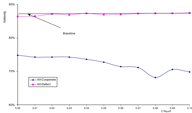
Figure 5: % Similarity versus C payoff, for all-coopering and all-defecting outcomes, \phi = 1 .
