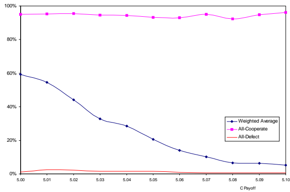
Figure 11: Welfare versus C payoff, for all-cooperating and all-defecting outcomes, \phi = 1 .
