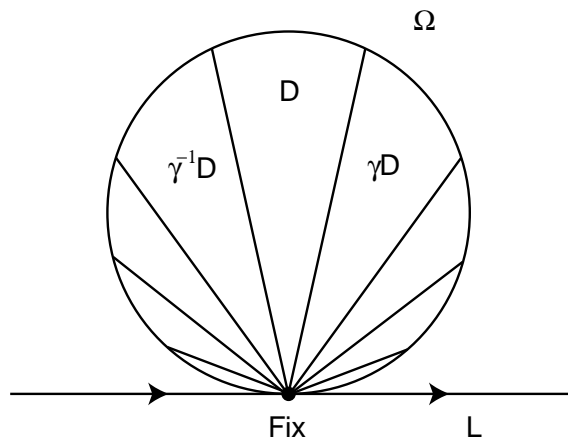
FIGURE 6. Parabolic Holonomy
